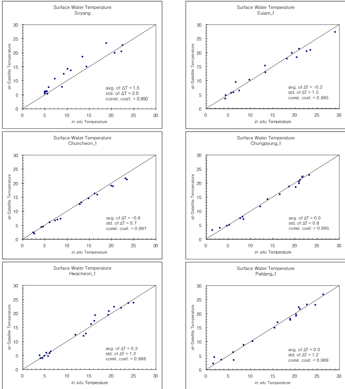
Fig 3. Relationship between the interpolated in situ and at-satellite water surface temperature ( T_{int\ p} and T_{sat}^{atmc} respectively) on each lake after applying statistical atmospheric correction
