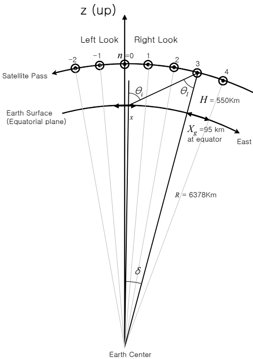
Fig. 2. Geometry of a satellite, a target, and the Earth.
