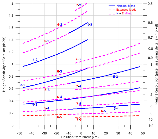
Fig. 6. The height sensitivity of parallax and the height resolution of radargrammetric image pairs as a function of the position from nadir. A pair of pass numbers is given on each line.
