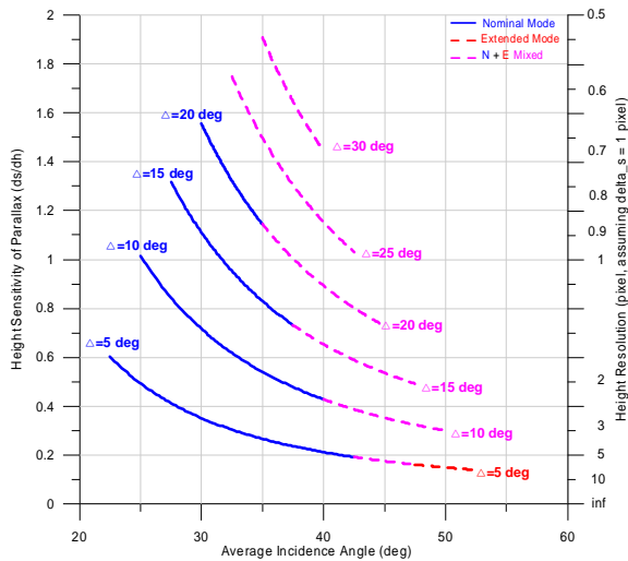
Fig. 5. The height sensitivity of parallax and the height resolution as a function of the average incidence angle. The delta is the difference of incidence angle between the radargrammetric image pair.
