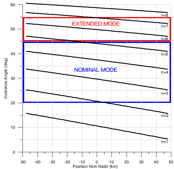
Fig. 3. Incidence angles as a function of the distance x from the nearest nadir. n is the pass number counted from the nearest nadir pass of a ground point.
