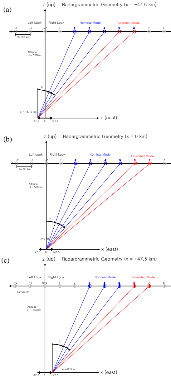
Fig. 4. Radargrammetric geometry of a point from adjacent passes. The ground point x is at (a) -47.5 km, (b) 0 km, and (c) 47.5 km away from the nadir.
