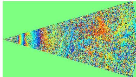
Fig. 8. Cross-Track InSAR, T3-T2, VV
