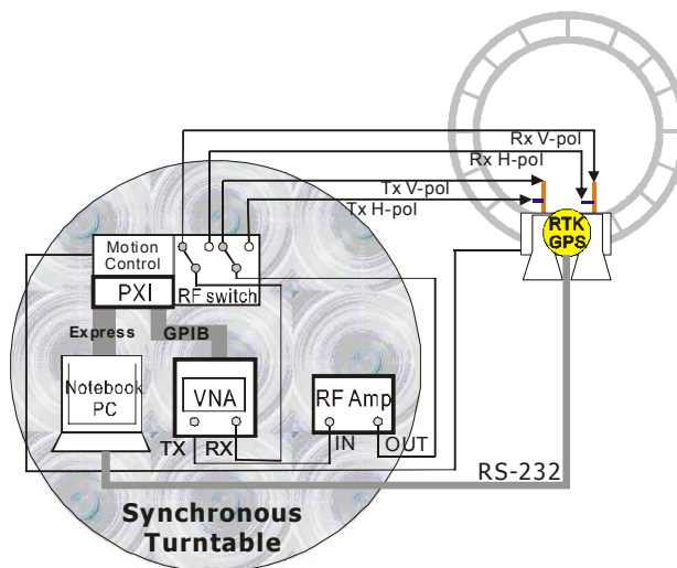
Fig. 2. Hardware configuration of an Arc-SAR
