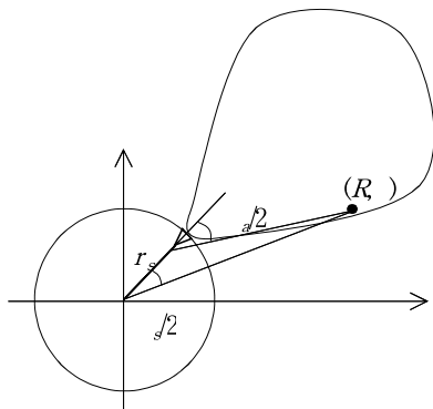
Fig. 3. Arc-SAR imaging geometry
