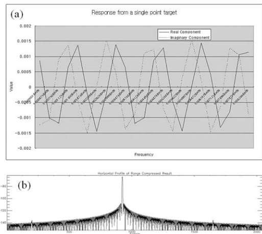
Fig. 3. (a) A part of the simulated raw signal for a point target. (b) Time domain signal generate by IDFT(Inverse Discrete Fourier Transform) of the simulated frequency domain signal shown in Fig. 3.
