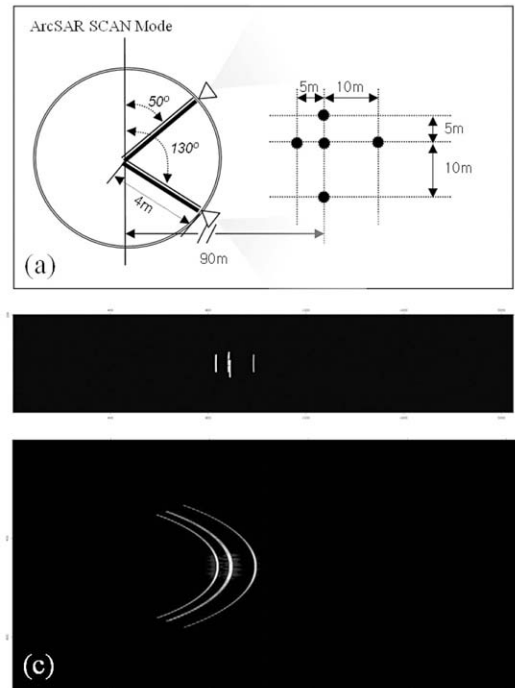
Fig. 6. (a) The schematic diagram of a model for the scan mode simulation which has 5 point targets, using a arc rail of 4m radius. (b) Range compressed result of the simulated raw signal. (c) Final ground based SAR image generated by azimuth compression using the conventional Deramp FFT technique.
