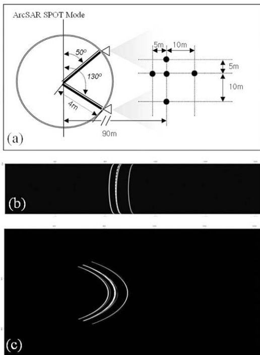
Fig. 7. (a) The schematic diagram of a model for the spot mode simulation which has 5 point targets, using a arc rail of 4m radius. (b) Range compressed result of the simulated raw signal. (c) Final ground based SAR image generated by azimuth compression using the conventional Deramp FFT technique.
