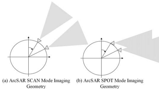
Fig. 2. Geometry of imaging system and spatial resolution of ground based SAR.
